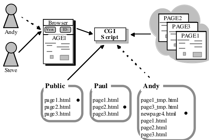
Figure 4 Supporting multiple authors
