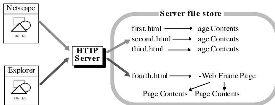
Figure 1. Replacement of existing web page with V-Web page
